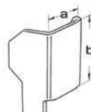
Dimensional Diagram
